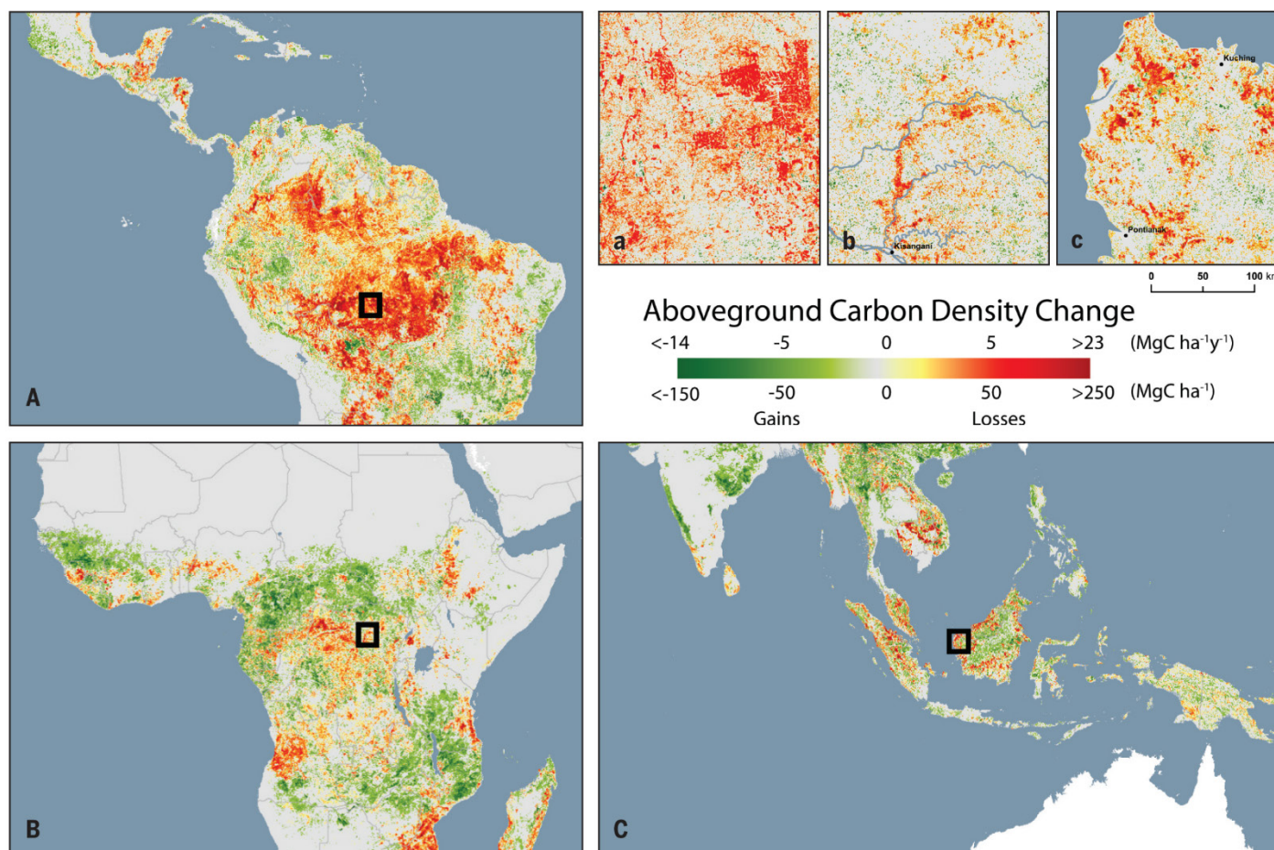
Fig. 1. Geography of carbon density change. The figure depicts the spatial distribution of areas exhibiting gains, losses, and no change (stable). Values reported are the change from 2003 to 2014 within each 463 × 463 m grid cell. Changes with a p-value larger than 0.05 are identified as stable. Data in panels A-C have been aggregated to 5 km for display. Insets a-c are shown at full resolution and correspond to the black rectangles in A-C, respectively.
